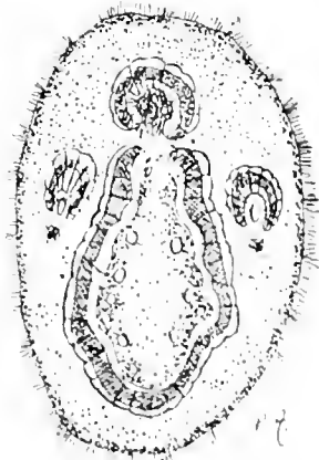
FIG. 30.— Shorea obtusa , Wall. Transverse section of internode below insertion of petiole, magnified 17 times. Three leaf traces in the bark, the apical with 3 resin ducts, each of the two lateral with one.
