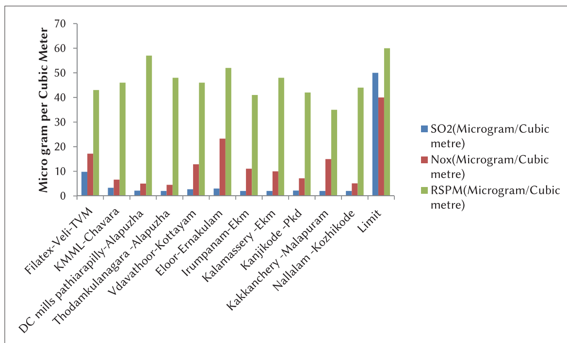
Figure 12.3 Annual average values of air pollutants at 11 monitoring stations in industrial areas of Kerala 2019
