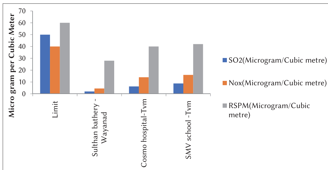
Figure 12.2 Annual average values of air pollutants at three monitoring stations in sensitive areas of Kerala 2019
