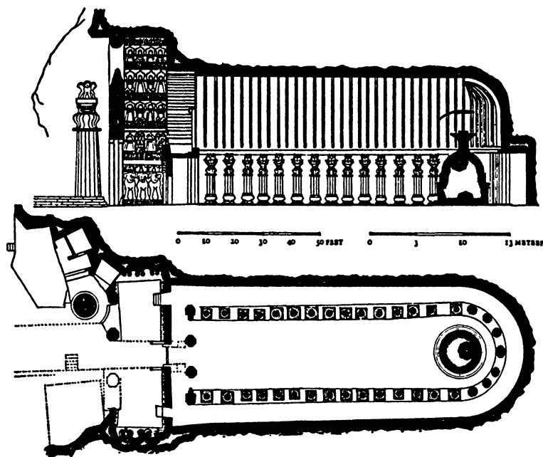
3. Chaitya hall at Karle: plan and elevation
