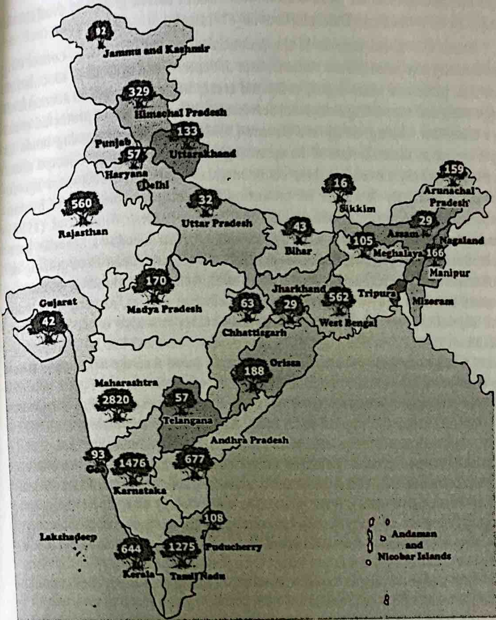
Figure 1. Distribution of sacred groves in India (after Kent, 2009).
